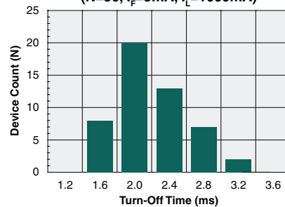
Typical Turn-Off Time (N=50, I_F=5\text{mA} , I_L=1000\text{mA} )
