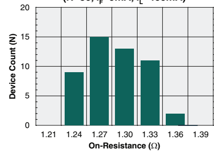
Typical On-Resistance Distribution (N=50, I_F=0\text{mA} , I_L=400\text{mA} )
