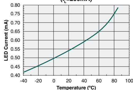
Typical I_F for Switch Operation ( I_L=200\text{mA} )
