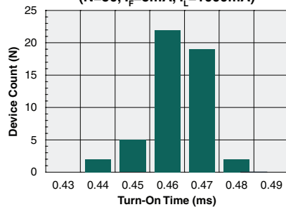
Typical Turn-On Time (N=50, I_F=5\text{mA} , I_L=1000\text{mA} )
