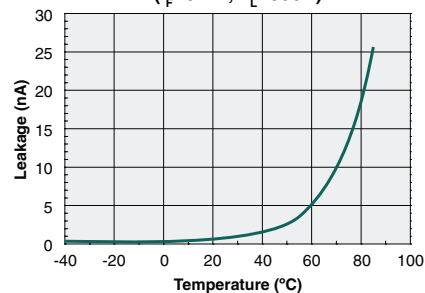
Typical Leakage vs. Temperature Measured Across Pins 3&4 ( I_F=0\text{mA} , V_L=350\text{V} )
