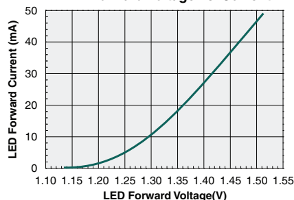
LED Forward Voltage vs. Current
