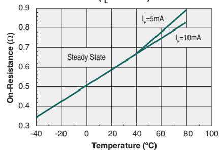
Typical On-Resistance vs. Temperature ( I_L=480\text{mA} )
