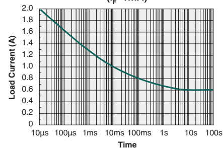
Energy Rating Curve ( I_F=1\text{mA} )
