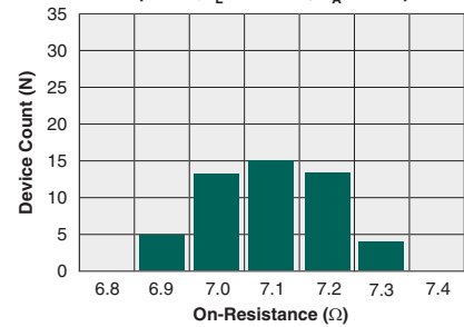
Typical On-Resistance Distribution (N=50, I_L=100\text{mA} , T_A=25^\circ\text{C} )
