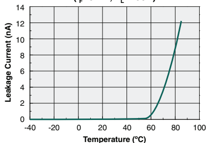
Typical Leakage vs. Temperature ( I_F = 0\text{mA} , V_L = 250\text{V} )
