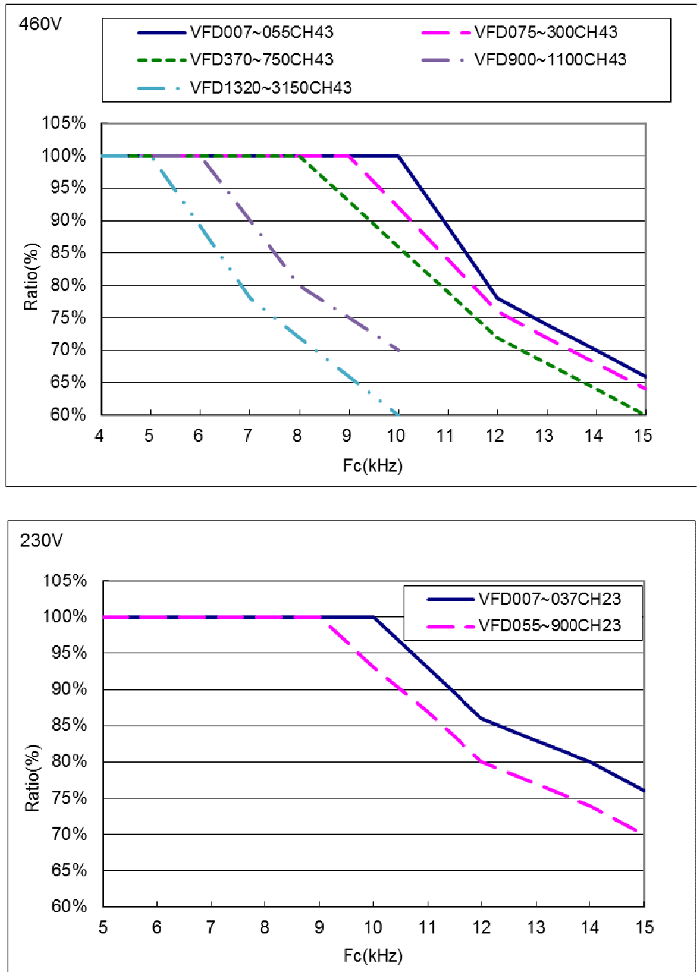
Figure 6.3.2-1 Load reduction curve of CH2000
