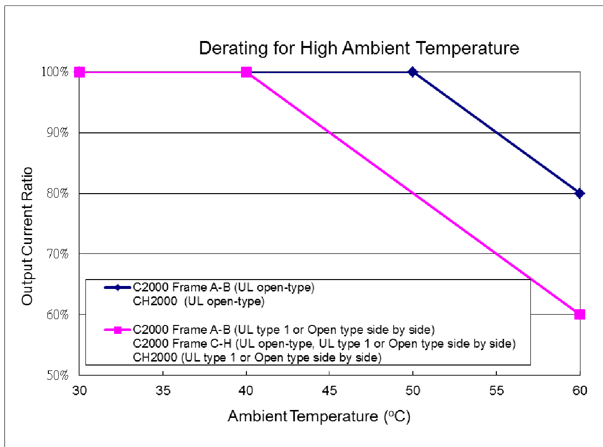
Figure 6.1.2 Environmental load reduction curve during advanced application
