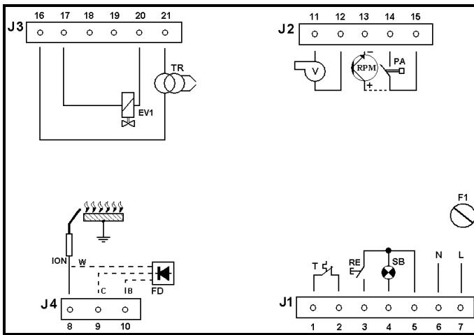
Type TGRD81
