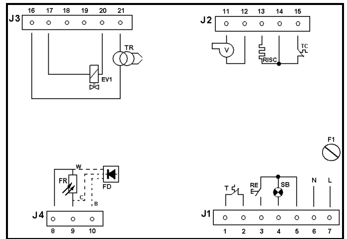
Type TGRD91
