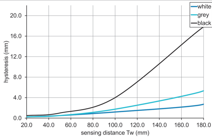
hysteresis curve
