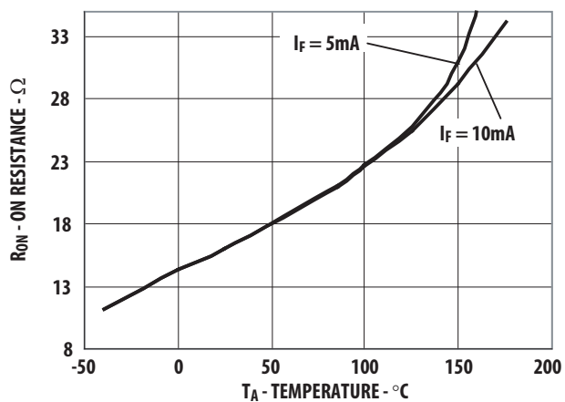
Figure 9: Typical On Resistance vs. Temperature
