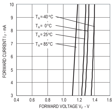
Figure 8: Typical Forward Current vs. Forward Voltage
