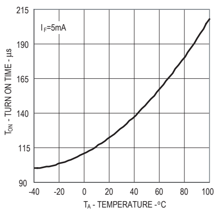
Figure 12: Typical Turn On Time vs. Temperature
