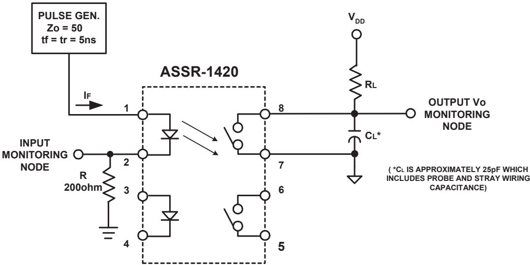
Figure 15: Switching Test Circuit for t_{ON} , t_{OFF}
