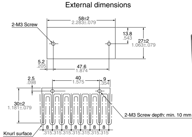
Heat sink attached to AQ1 relay
