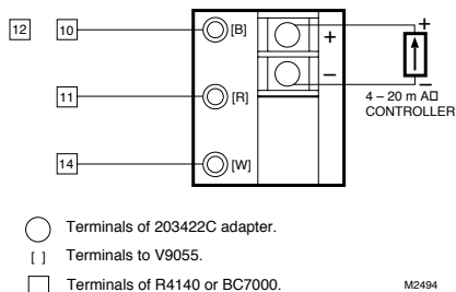
Fig. 1—Hookup of V9055 for firing rate control with 4-20 mA input.
