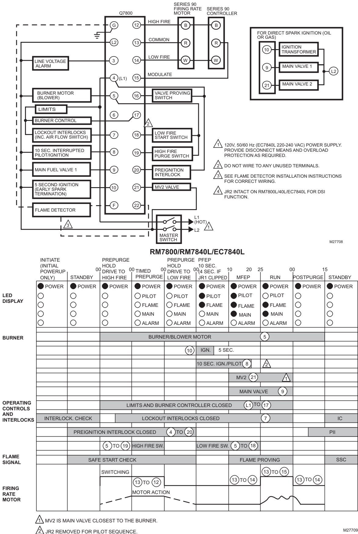
Fig. 4. Wiring subbase and sequence for RM7800L/40L, EC7840L with Valve Proving feature enabled.
