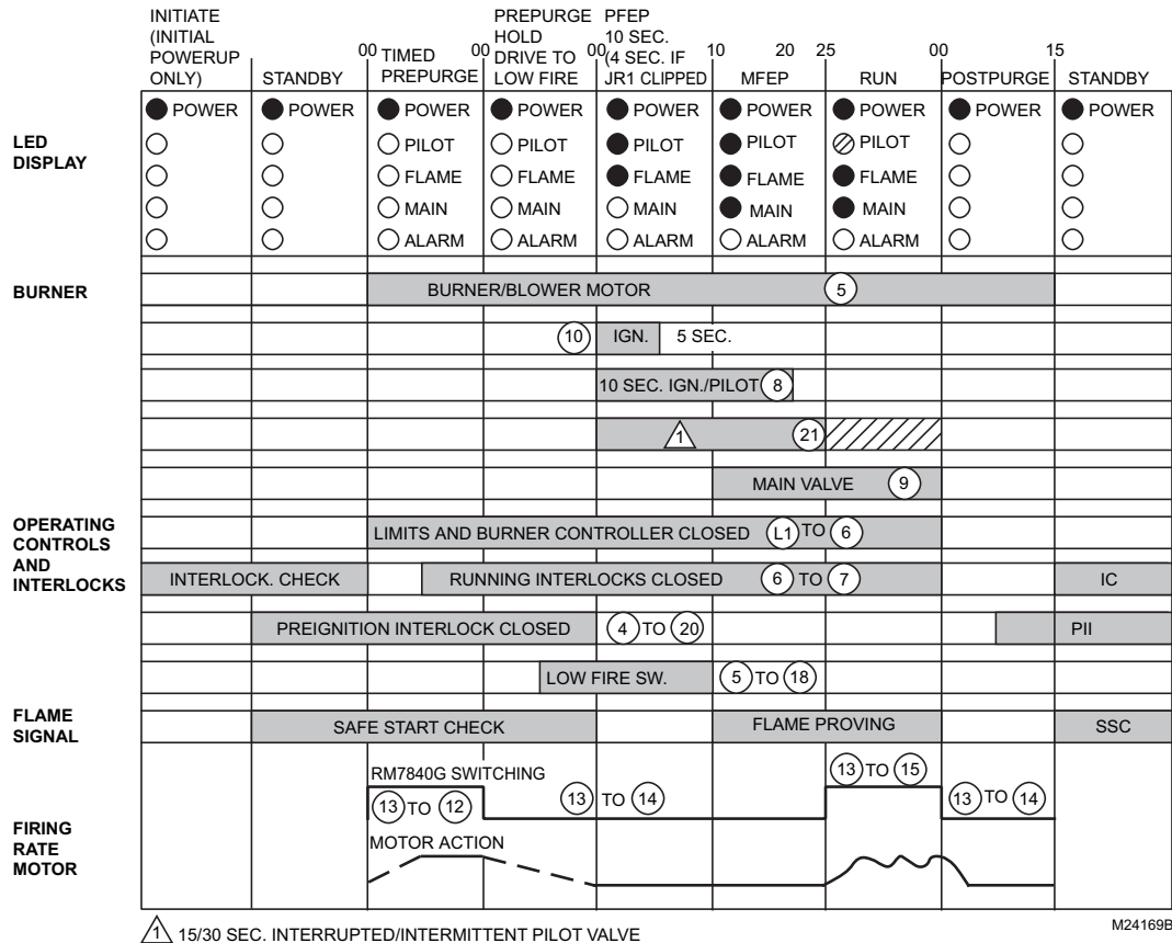
Fig. 6. Typical wiring subbase and sequence for RM7840G without Valve Proving enabled.
