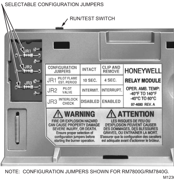
Fig. 27. Selectable site-configurable jumpers.
