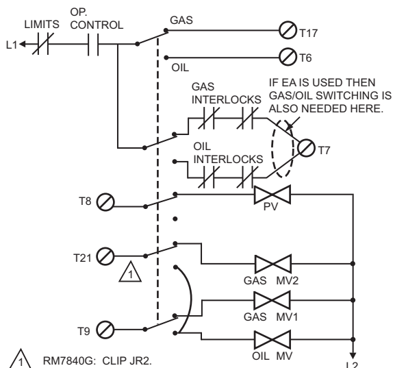
1 RM7840G: CLIP JR2 AND JR3. P. VALVE PROVING/DUAL FUEL: GAS 10 SECOND MFEP, OIL 15 SECOND MFEP M24133B
