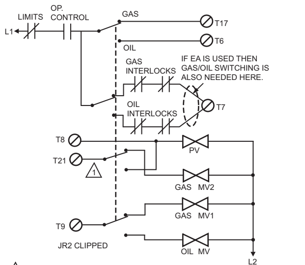
1 RM7840G: CLIP JR2 AND JR3. P. VALVE PROVING/DUAL FUEL: GAS 10 SECOND MFEP, OIL 15 SECOND MFEP M24133B
