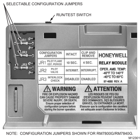
Fig. 27. Selectable site-configurable jumpers.
