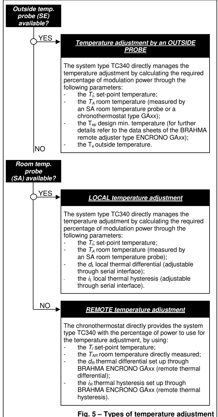
Fig. 5 – Types of temperature adjustment
