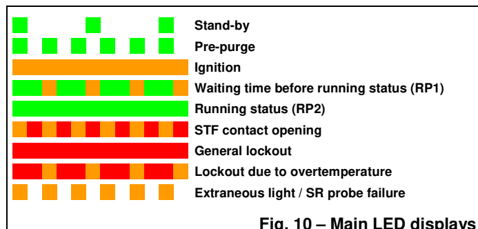
Fig. 10 – Main LED displays
