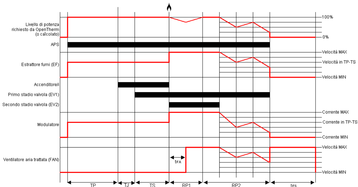
TC340(A-P) – Standard operating cycle using BRAHMA chronothermostat type ENCRONO GAxx
