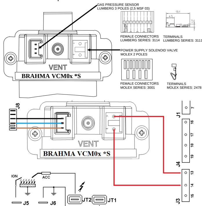
Fig. 5.c – Connections and wiring diagram of VCMxx *S.
