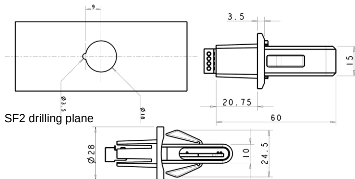
Fig. 5.f – Dimensions and fixing of SF2 sensors
