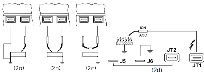
Fig. 2 – Inbuilt Ignition device connections
