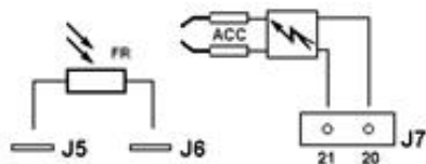
Fig.4a-Type, fixing systems and connections of FT, FC sensors
