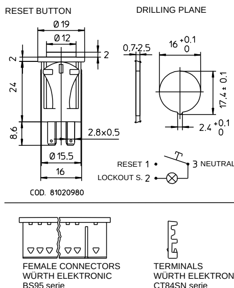
Fig. 4 – Standard accessories
