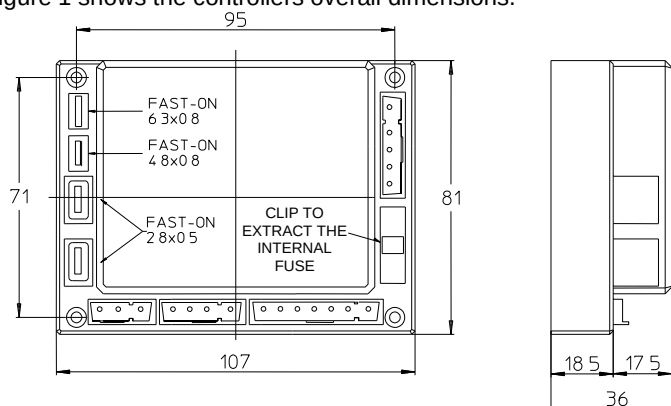
Fig. 1 – Overall dimensions
