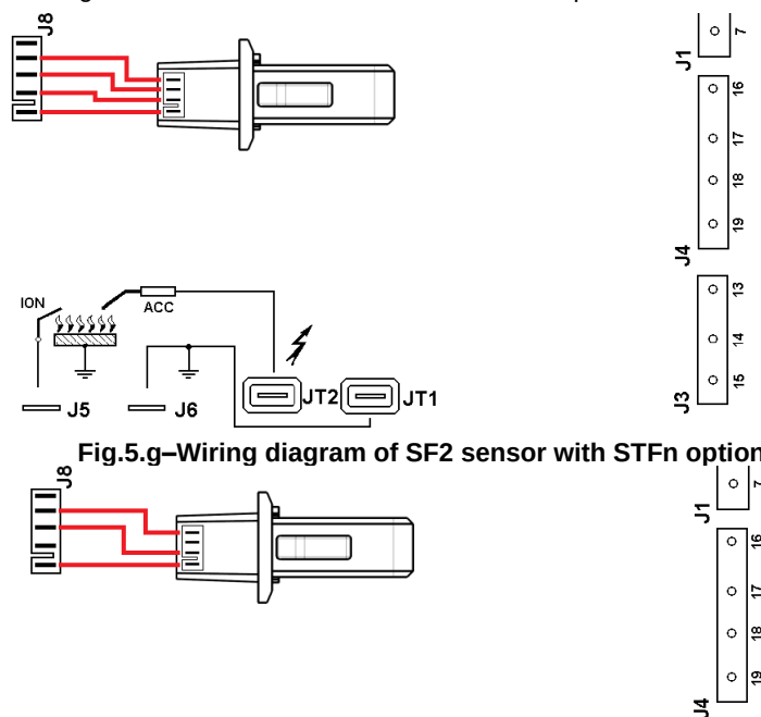
Fig. 5.g – Wiring diagram of SF2 sensor with STFn option
