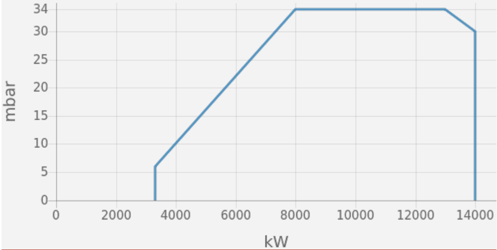
WORKING DIAGRAM
