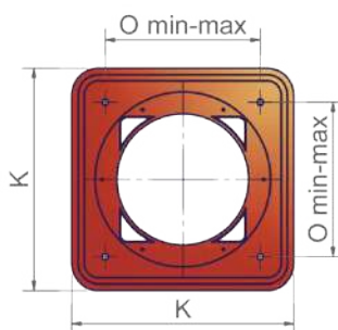
BURNER FLANGE
