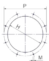
BOILER RECOMMENDED DRILLING TEMPLATE
