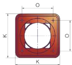
BURNER FLANGE
