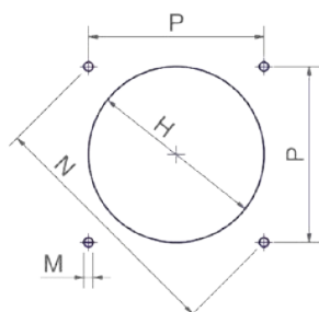
BOILER RECOMMENDED DRILLING TEMPLATE
