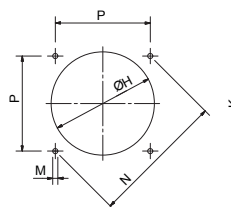
BOILER RECOMMENDED DRILLING TEMPLATE
