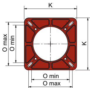
BURNER FLANGE
