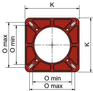
BURNER FLANGE
