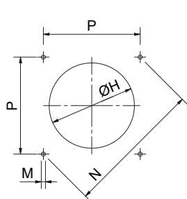
BOILER RECOMMENDED DRILLING TEMPLATE
