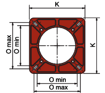
BURNER FLANGE
