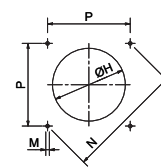
BOILER RECOMMENDED DRILLING TEMPLATE
