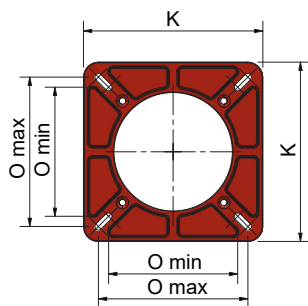
BURNER FLANGE
