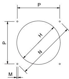
BOILER RECOMMENDED DRILLING TEMPLATE
