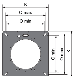
BURNER FLANGE
