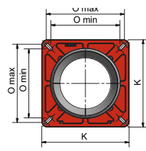
BURNER FLANGE
