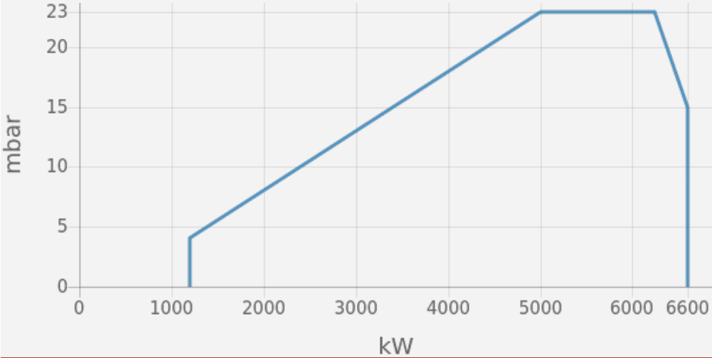
WORKING DIAGRAM
